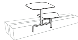
art. 4242 cm 69x45x50,5h (cm 50,5h su trave/on beam)
